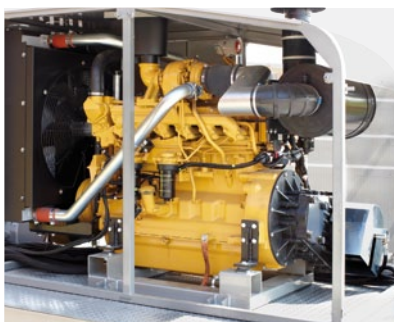
Independent unit with John Deere engine (250 HP)
